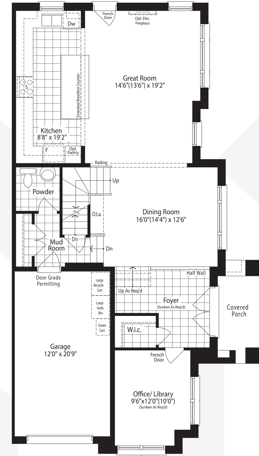
First Floor Elevation B
