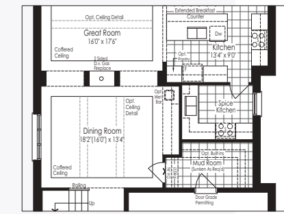
Optional First Floor With Spice Kitchen
