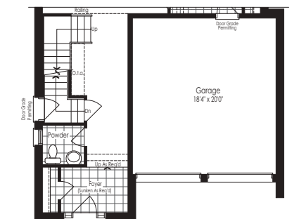
First Floor Elevation C
