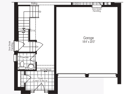
First Floor Elevation B
