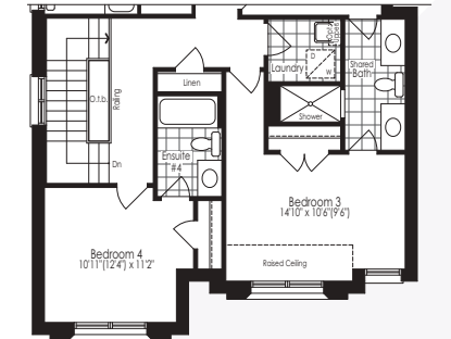
Opt. 5 Bedroom Second Floor Elevation C
