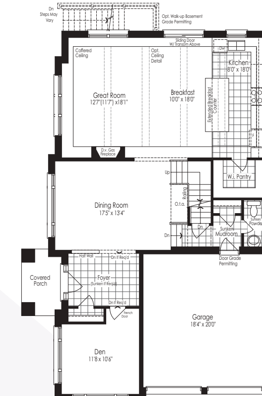
First Floor - Elevation B
