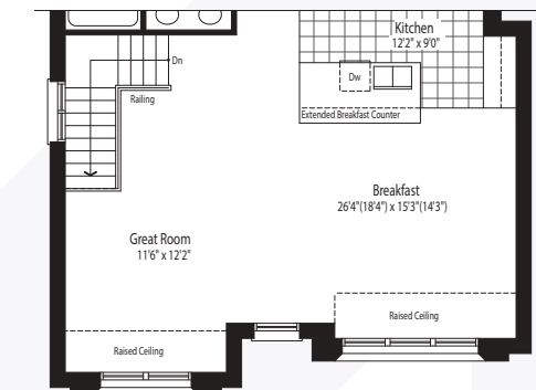
Second Floor Elevation C
