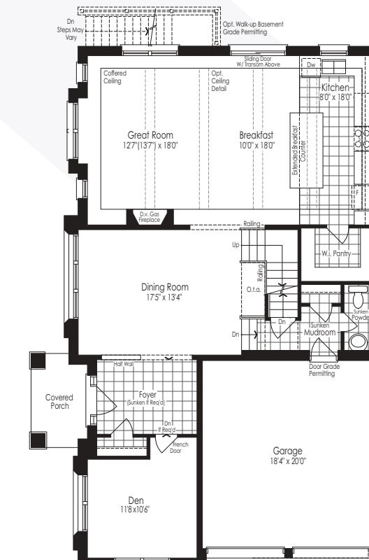
First Floor - Elevation C
